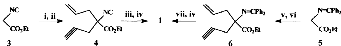
Scheme 2: i. Allyl bromide, n\text{-Bu}_4\text{NHSO}_4 , \text{K}_2\text{CO}_3 ii. propargyl bromide, n\text{-Bu}_4\text{NHSO}_4 , \text{K}_2\text{CO}_3 iii. HCl, EtOH iv. \text{Ag}_2\text{O} , DMAP, \text{CH}_2\text{Cl}_2 v. propargyl bromide, \text{K}_2\text{CO}_3 vi. allyl bromide, KOH, n\text{-Bu}_4\text{NBr} vii. 1N HCl, ether
